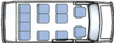
Optional 12-passenger seating with rear luggage compartment shown with flip-up cargo door seat
